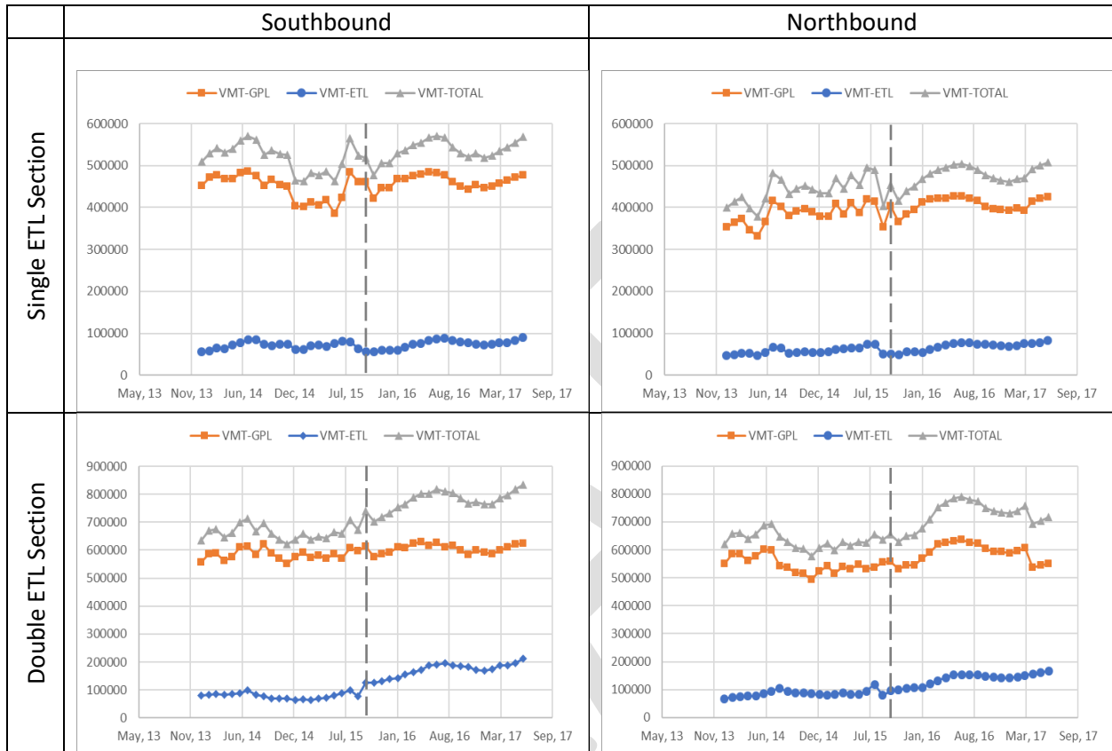
Figure 10. Average daily VMT for the 42-month study period separated by direction, ETL sections, and lane types
