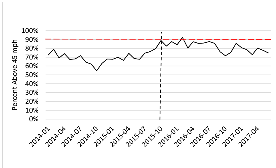
Figure 19: Percent time in peak hour with southbound ETL speed above 45 mph
