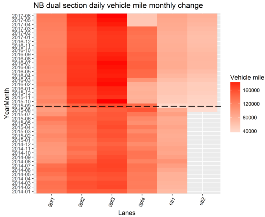
Figure 12. Northbound lane-by-lane average daily vehicle-miles for the study period, separated by dual and single sections
