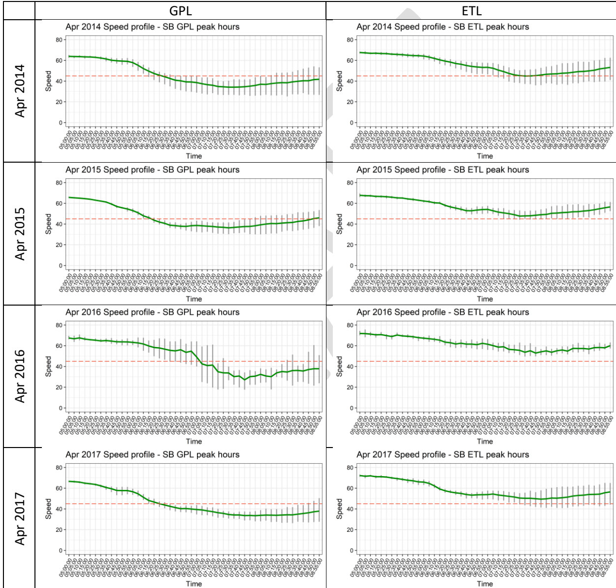
Figure 17. Speed profiles in the southbound ETL and GPL in the peak period for the month of April 2014-2017
