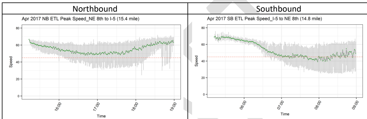
Figure 20. Peak speed profiles in the ETL for April 2017
