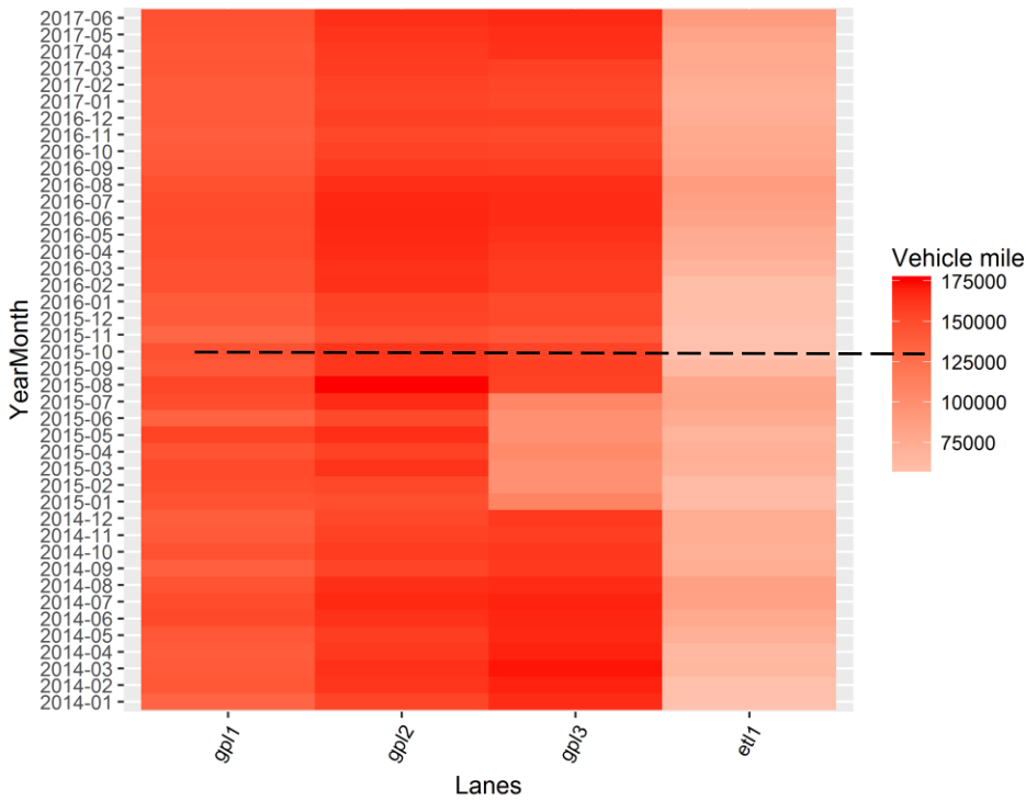
SB single section daily vehicle mile monthly change
