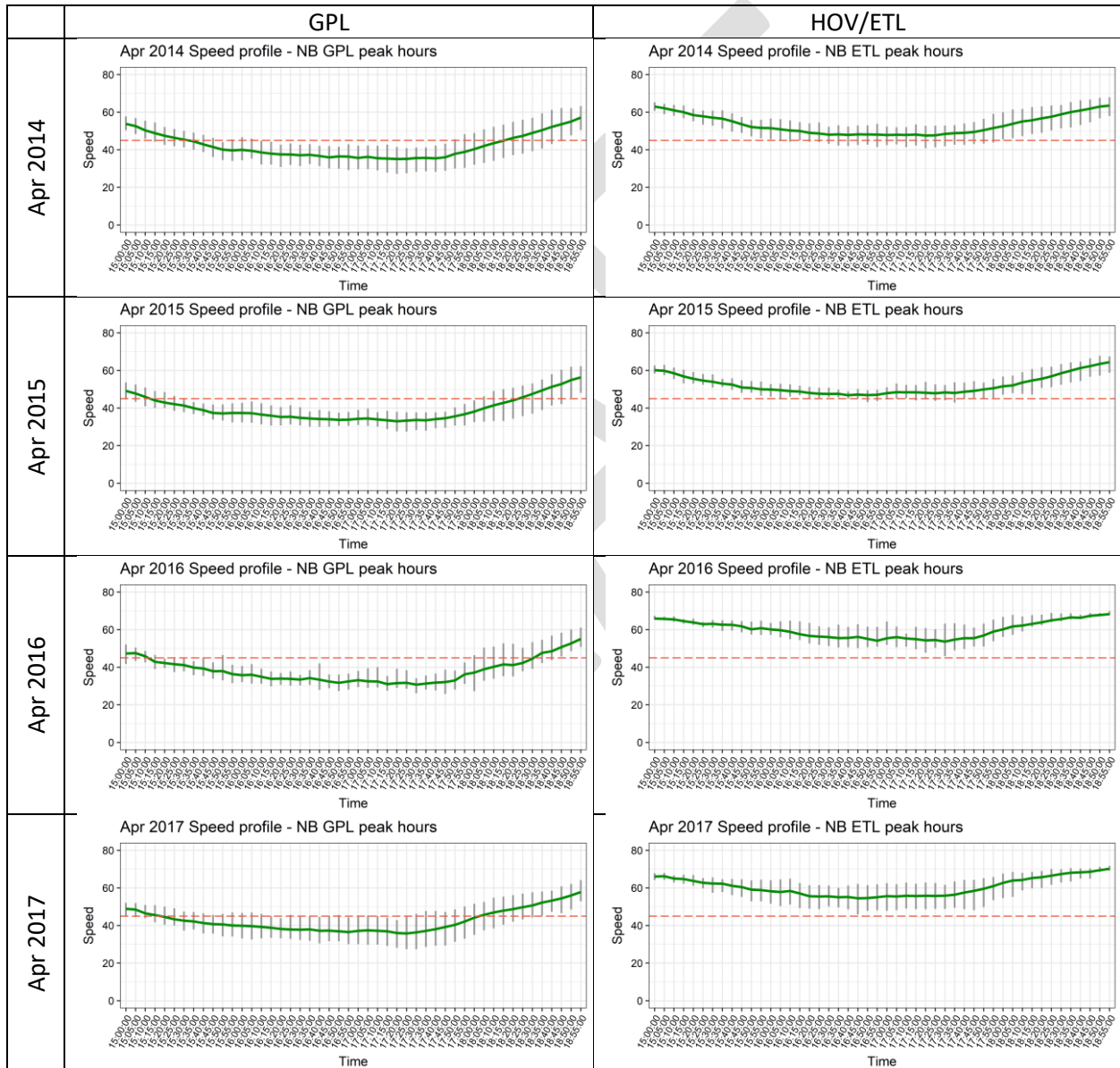
Figure 16. Speed profiles in the northbound ETL and GPL in the peak period for the month of April 2014-2017
