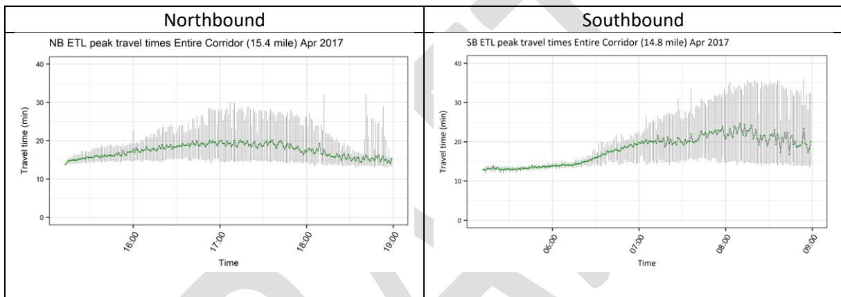
Figure 9. Peak travel time profiles in the ETL for April 2017.
